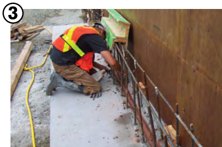
3 Create two levels of construction joint protection with both a physical and crystalline chemical barrier by using the Krystol® Waterstop System.
