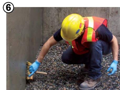
Waterproof where existing membranes have failed or where there was no initial waterproofing with Krystol T1 & T2®; a cementitious slurry system that becomes an integral part of the concrete to prevent water ingress.
