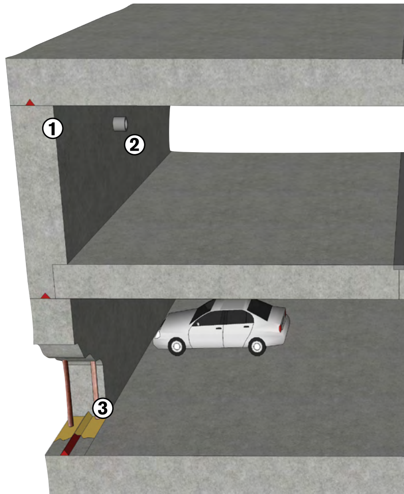
1 Create a watertight structure by using Krystol Internal Membrane™ (KIM®) in precast, cast-in-place or shotcrete walls and slabs. KIM builds the waterproofing right in to the concrete, eliminating the need for unreliable membranes.
