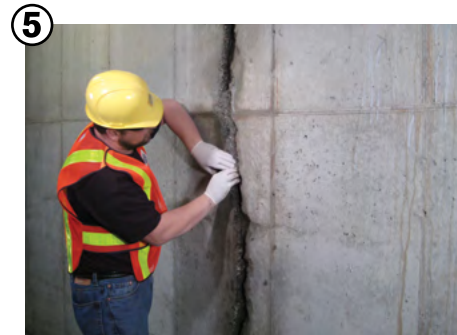
Waterproof leaking cracks and joints using the Krystol Leak Repair System.
